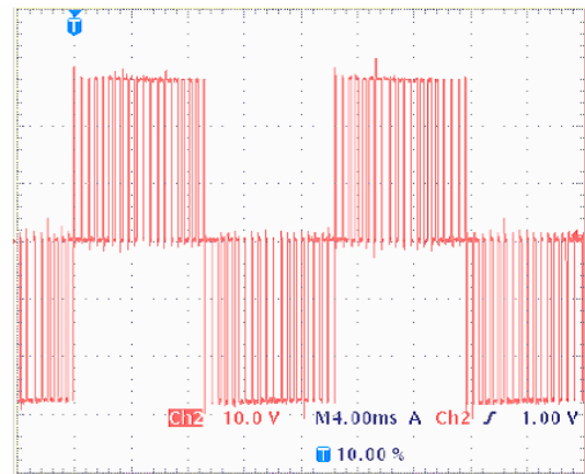
Fig.11 Unfiltered output voltage five levels at Ma=0.4
