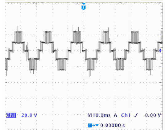
Fig.10 Unfiltered output voltage five levels at Ma=0.8
