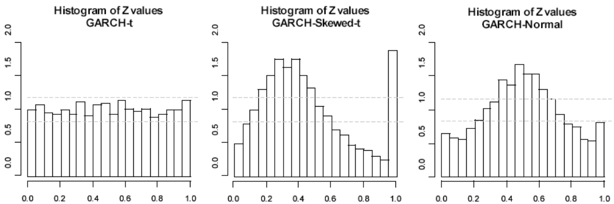
FIGURE 2. Comparison of the PIT histograms (GARCH model)
