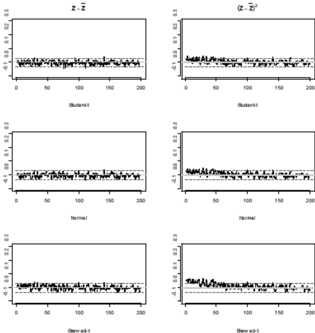
FIGURE 3. Autocorrelation of z - \bar{z} and (z - \bar{z})^2 from GARCH(1,1)
