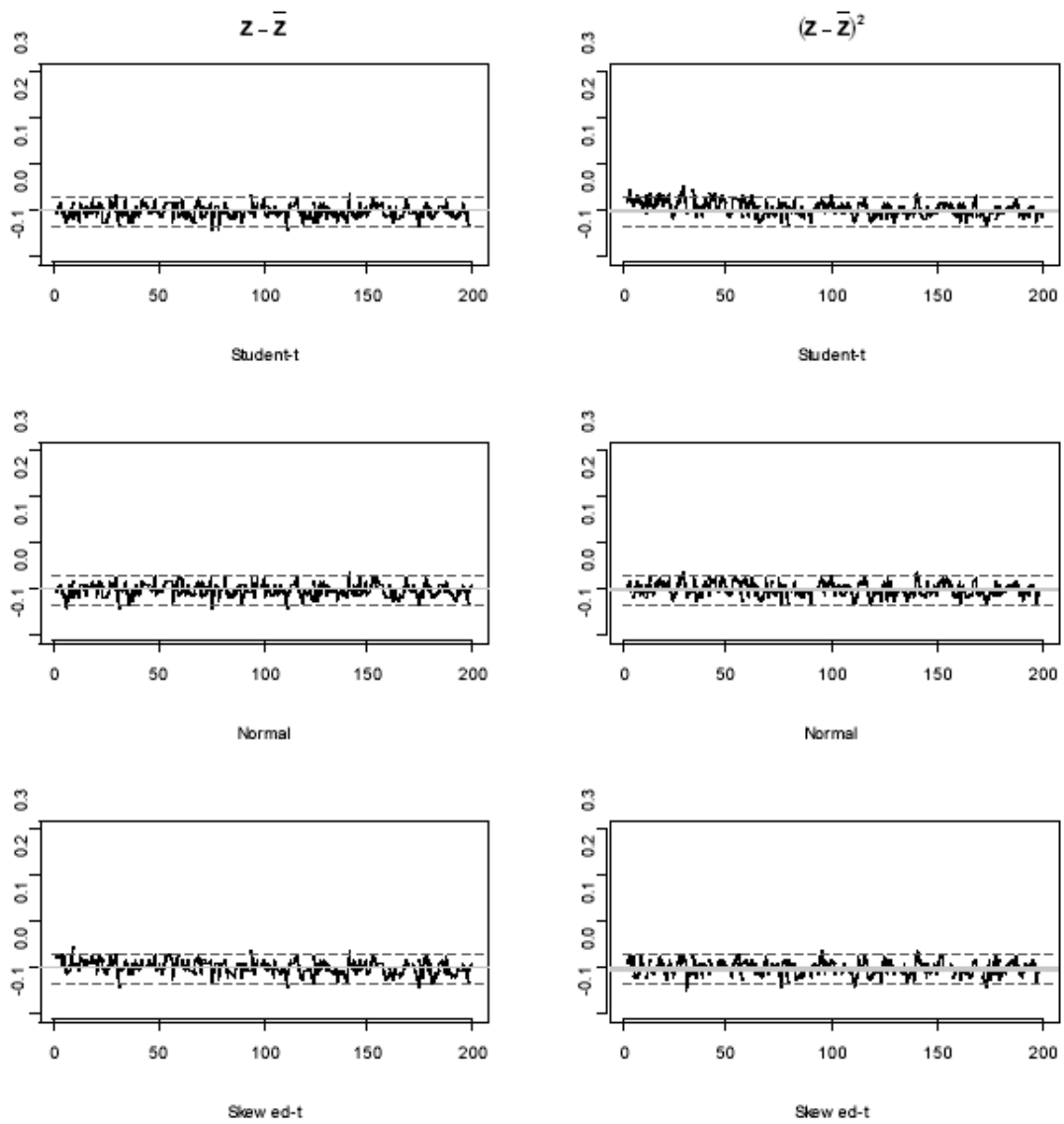
FIGURE 5. Autocorrelation of z - \bar{z} and (z - \bar{z})^2 from EGARCH(1,1)
